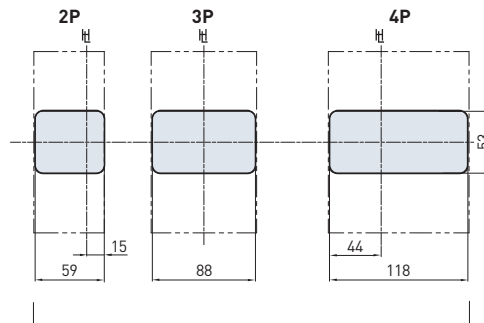
[Panel cut-out]
