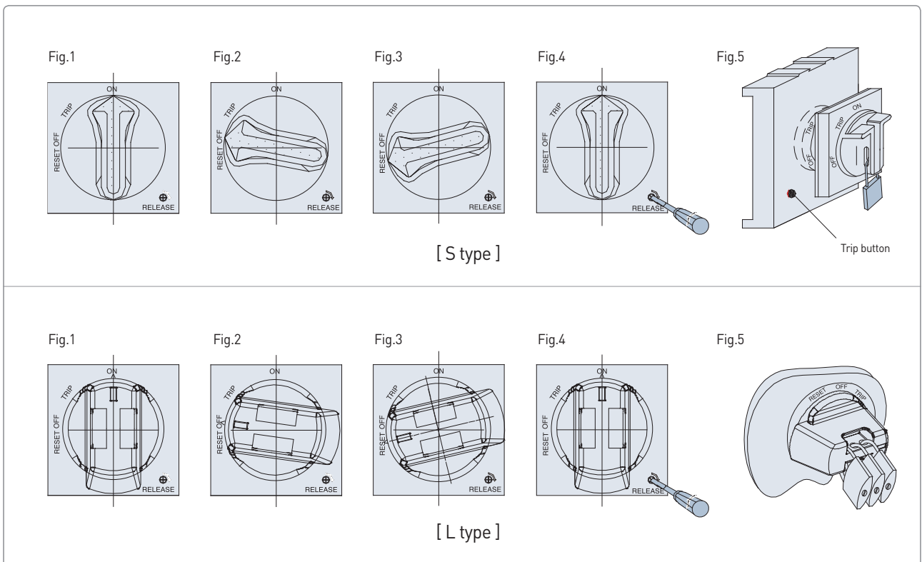
ON, OFF and TRIP are not marked on real products.
