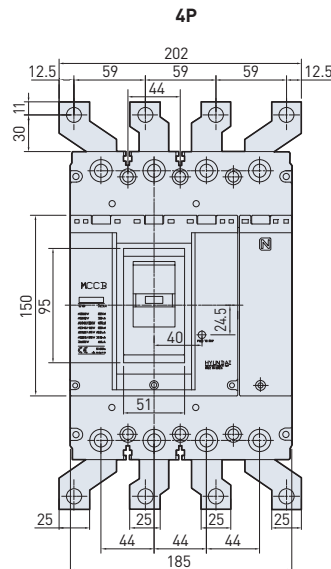
[Connection conductor]
