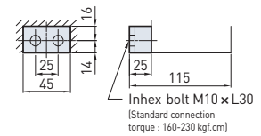
[Terminal part]
