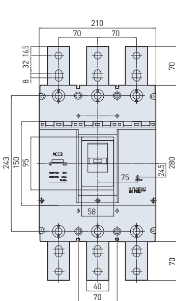
[Terminal part]
