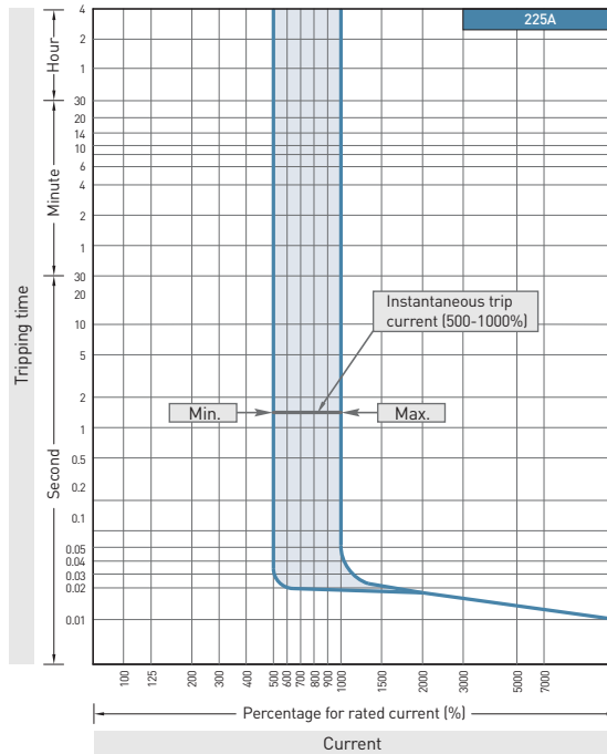
Tripping curves
